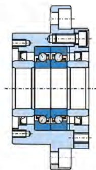
Fig. 9 Ball screw support bearing units
