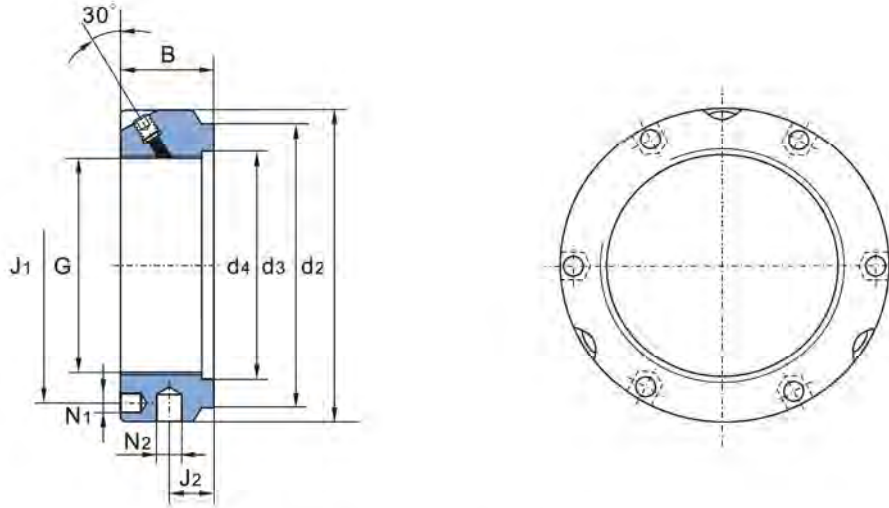
KMB-type locknuts
