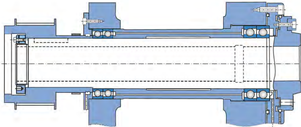
Fig. 24 Super-speed CNC lathe spindle
