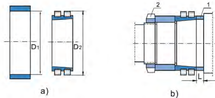
Fig. 23 Mounting cylindrical roller bearings
