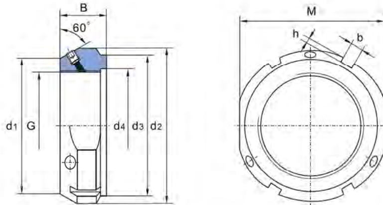
KMA-type locknuts
