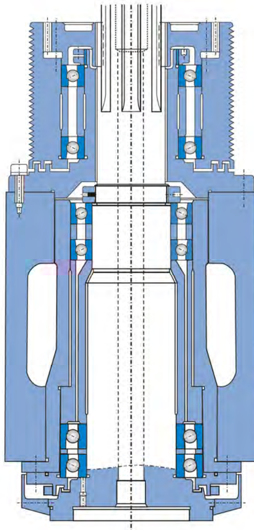
Fig. 25 Vertical lathe spindle
