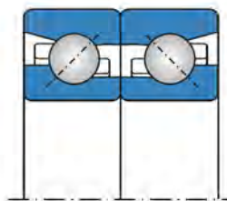
Fig. 4 High-speed angular contact thrust ball bearing structure
