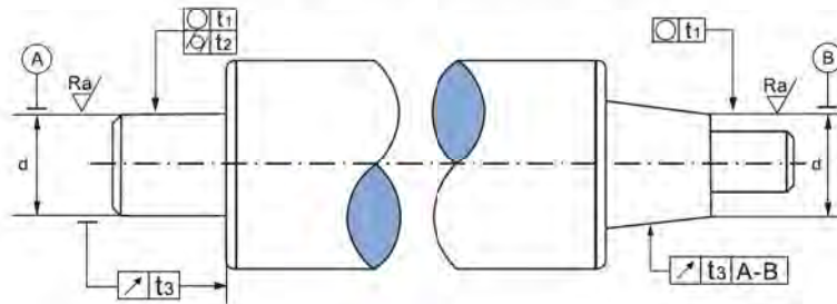
Fig. 16 Fitting tapered shaft
