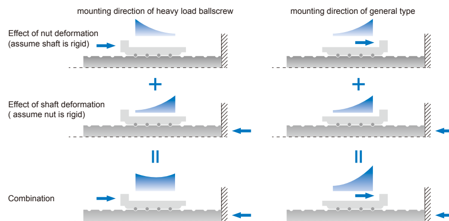
Fig.8 Load distribution
