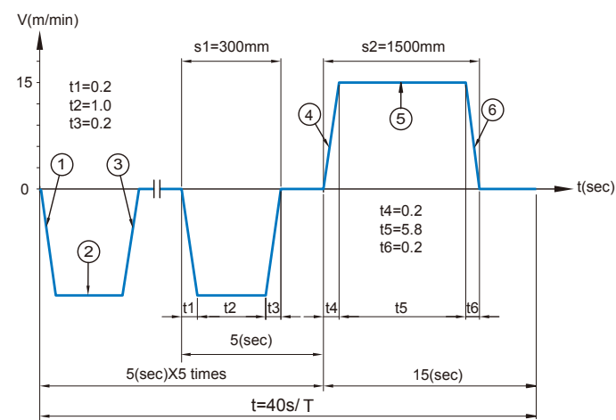
Fig.37 Porterage apparatus v-t diagram
