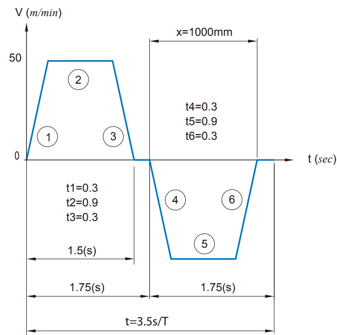
Fig.35 Portorage apparatus v-t diagram
