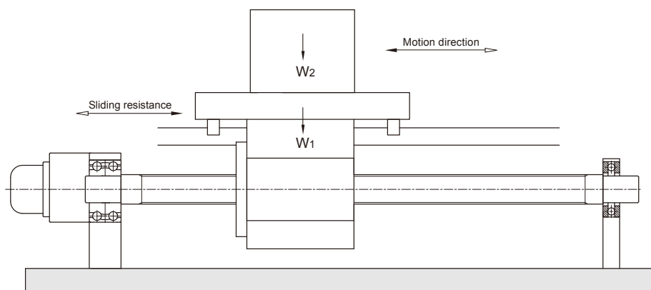
Fig.34 High speed portorage apparatus
