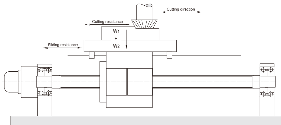
Fig.33 Cutting machine
