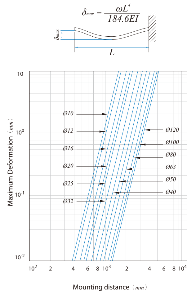
Fig.14 Maximun deformation for fixed-supported
