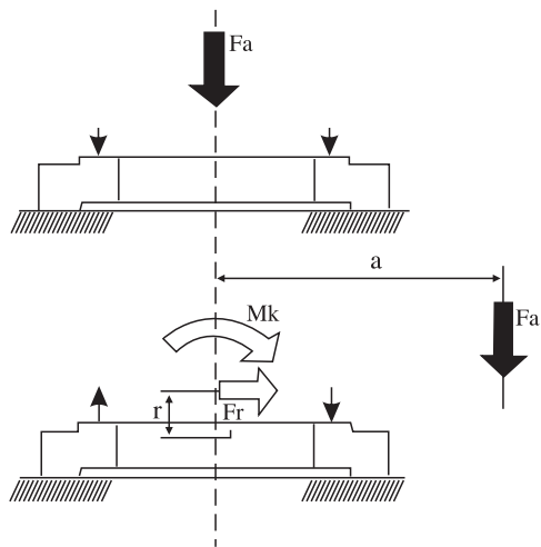
图 1：转盘轴承通常安装在支承结构上面 Fig. 1: Slewing bearings are generally installed on the supporting structure
