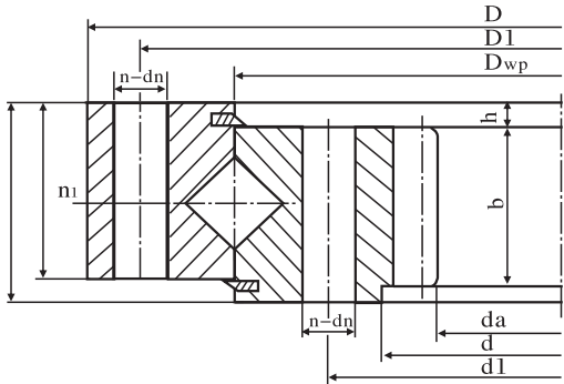
内齿式交叉圆柱滚子轴承 ( 113, 114 ) Cross Roller Bearing with Inner Gear
