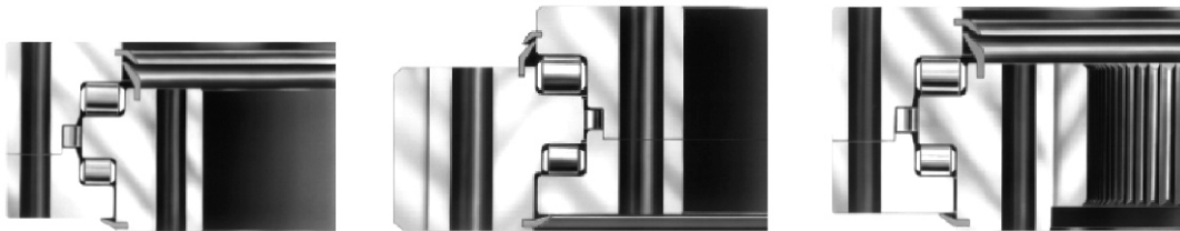
三排圆柱滚子组合转盘轴承 Three row cylindrical roller slewing bearing
