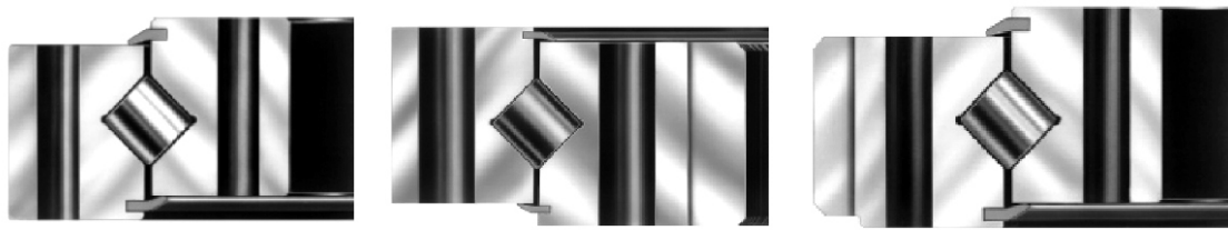
单排交叉滚子转盘轴承 Single row cross roller slewing bearing
