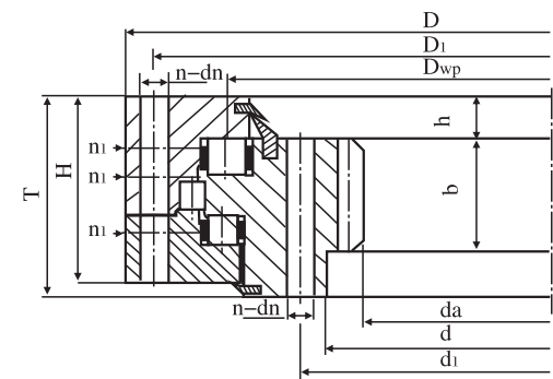
内齿式三排圆柱滚子组合轴承 (133, 134) With Inner Gear
